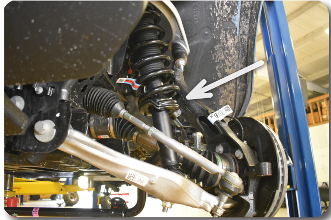
Figure 13C (Driver Side viewed from the front)
