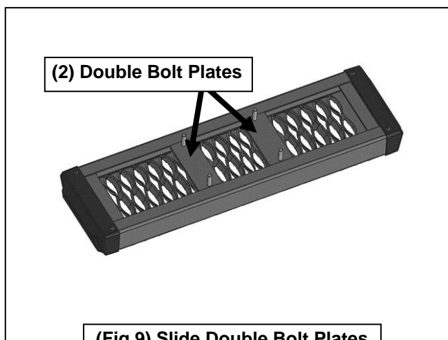
(Fig 9) Slide Double Bolt Plates into channel on bottom of Step
