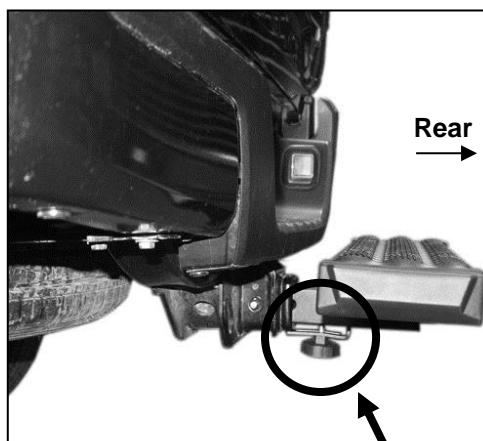
(Fig 8) Anti-rattle Bracket attached to Bar Welded Bracket
