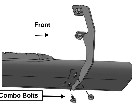
(Fig 6) Sidebar attached to Mounting Bracket
