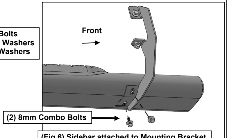
(Fig 6) Sidebar attached to Mounting Bracket
