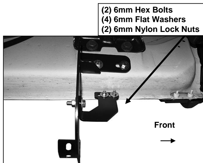
(Fig 13) Driver side front Bracket assembly
