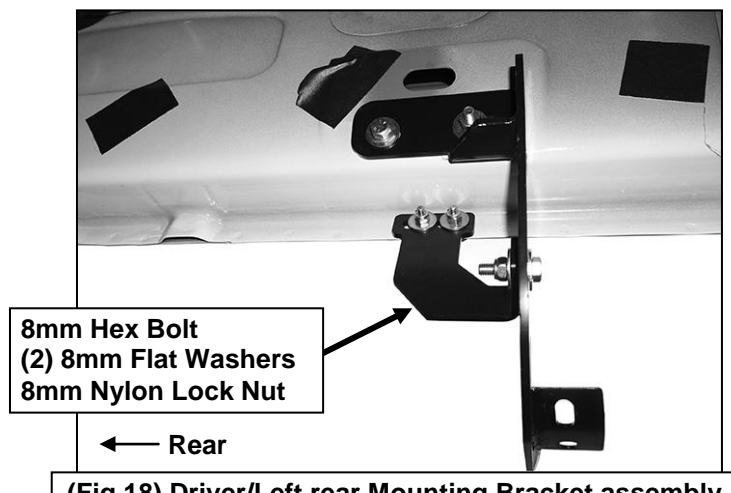
(Fig 18) Driver/Left rear Mounting Bracket assembly
