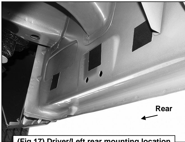
(Fig 17) Driver/Left rear mounting location
