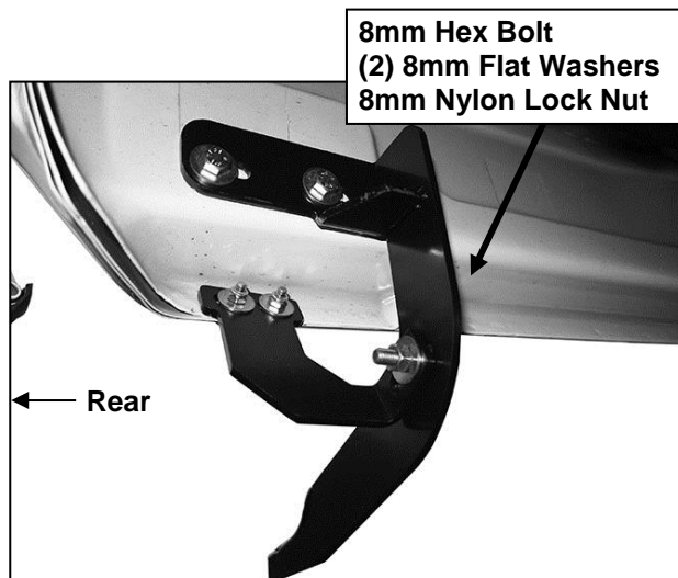
(Fig 18) Driver/Left rear Mounting Bracket assembly
