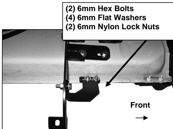
(Fig 13) Driver side front Bracket assembly
