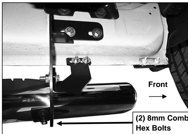
(Fig 19) Driver/Left front Mounting Brackets
