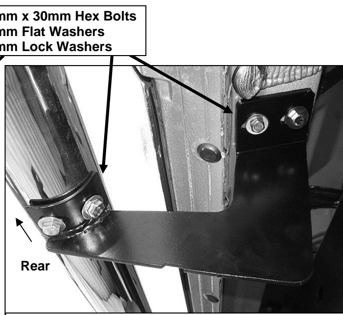
(Fig 4) Driver side rear mounting location pictured
