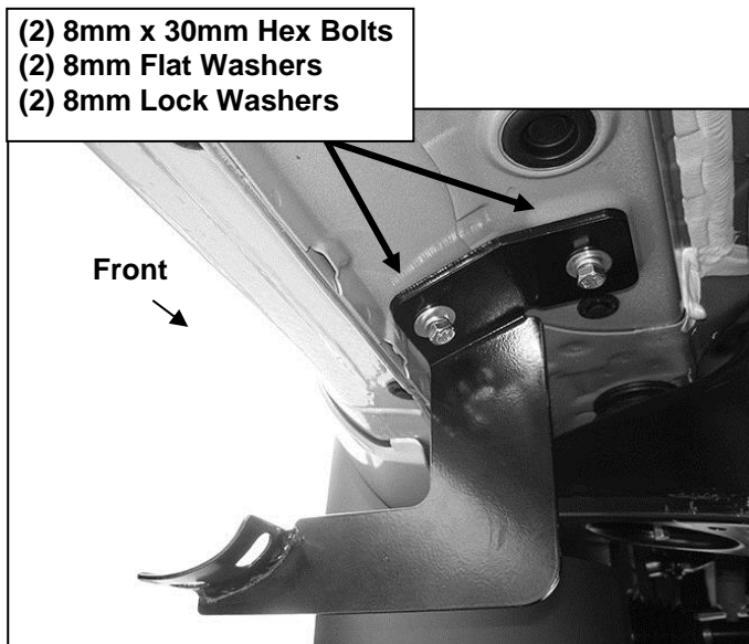
(Fig 2) Driver side front mounting location pictured
