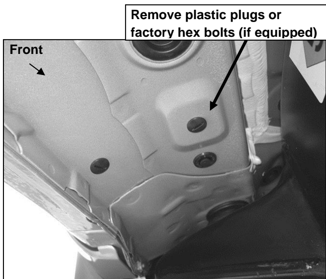
(Fig 1) Driver side front mounting location pictured
