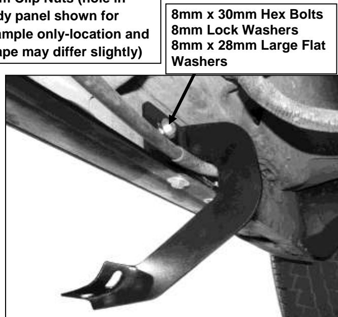
(Fig 2) Driver side-front Mounting Bracket location
