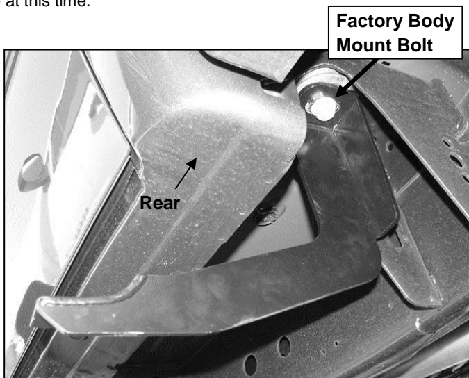
(Fig 2) Rear Mounting Bracket installation pictured
