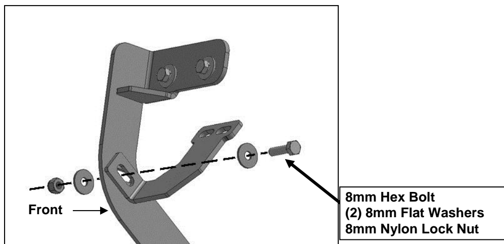
(Fig 11) Attach Driver/Left front Support Bracket to front facing side of Mounting Bracket
