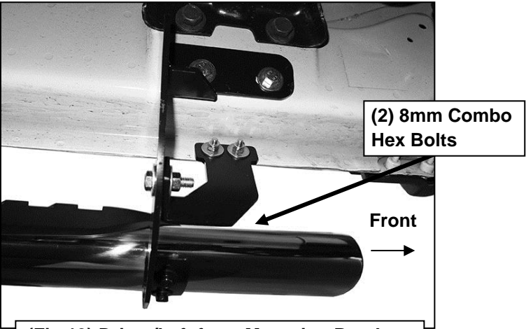
(Fig 19) Driver/Left front Mounting Brackets
