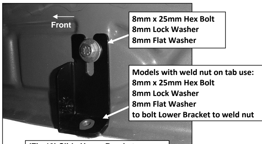
(Fig 13) Slide Upper Bracket over weld nut (if equipped-see Figure 2)
