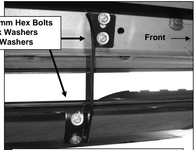
(Fig 4) Driver/Left Center Bracket Pictured
