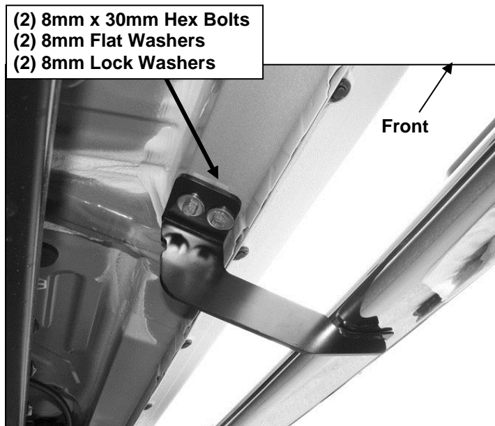
(Fig 3) Driver side center mounting location pictured
