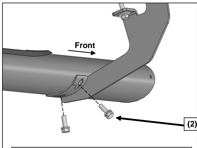
(Fig 5) Sidebar attached to Mounting Bracket
