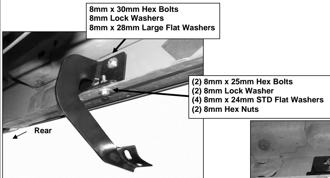
(Fig 3) Driver side-rear Mounting Bracket location
