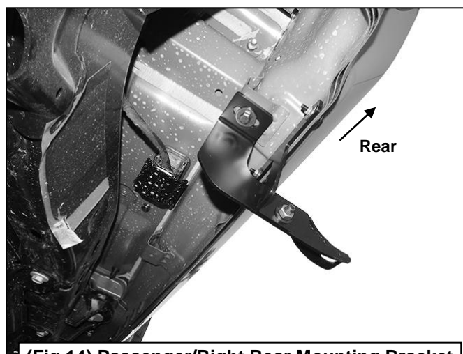
(Fig 14) Passenger/Right Rear Mounting Bracket and Support Bracket attached to rear location
