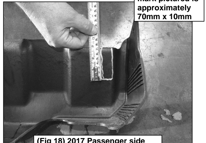
(Fig 18) 2017 Passenger side DEF cover marked for trimming
