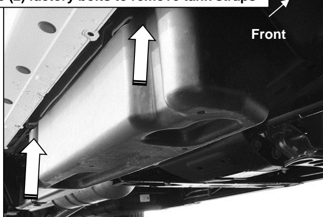
(Fig 11) 07-16 Passenger side DEF tank and cover
