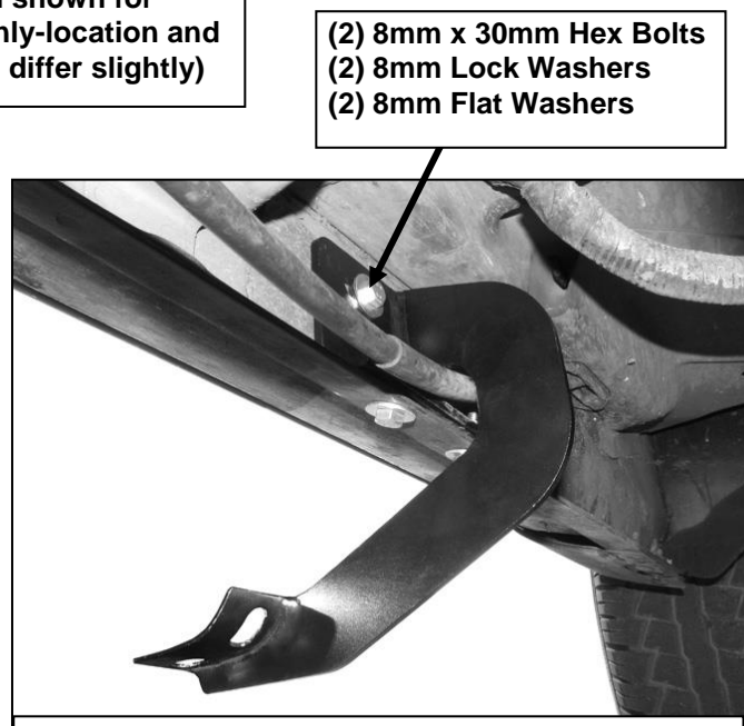
(Fig 2) Driver side-front Mounting Bracket location
