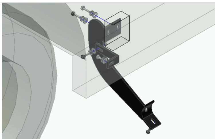
Figure 1.2 - Front Bracket
