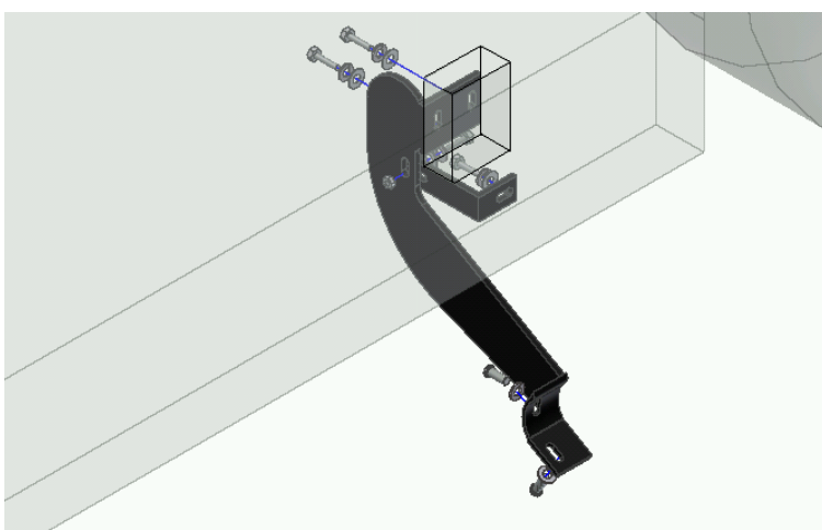
Figure 1.3 - Rear Bracket
