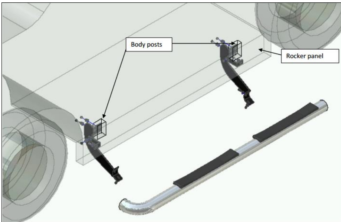
Figure 1.2 - Front Bracket
