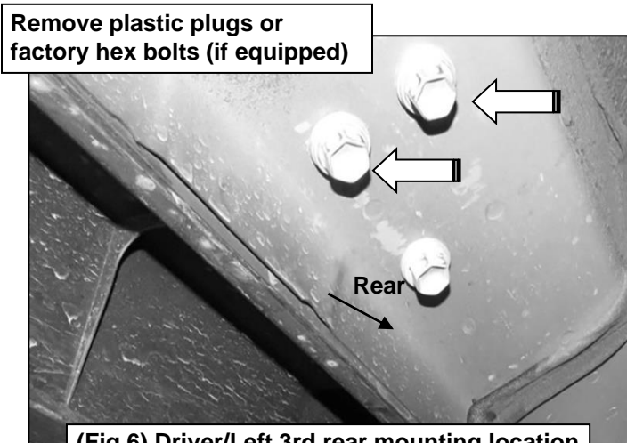
(Fig 6) Driver/Left 3rd rear mounting location
