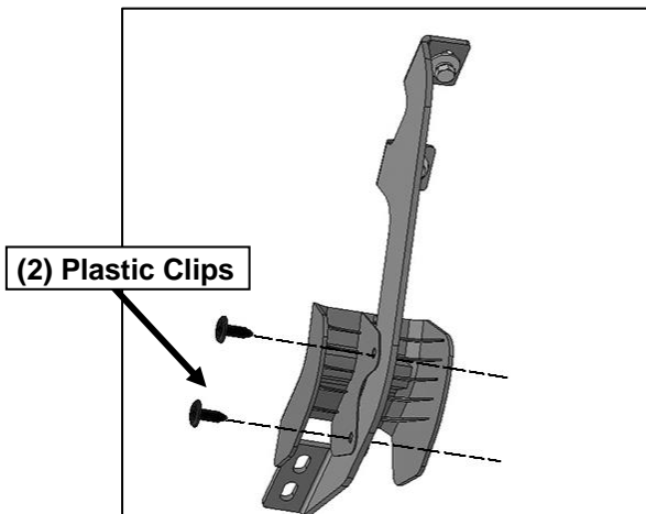
(Fig 3) Attach (1) Plastic Cover to the Mounting Bracket with (2) Plastic Clips
