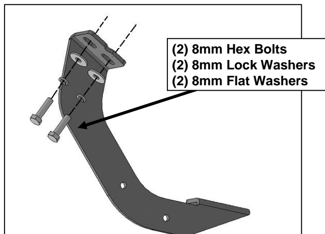
(Fig 5) Attach Driver/Left Center Mounting Bracket to the floor panel
