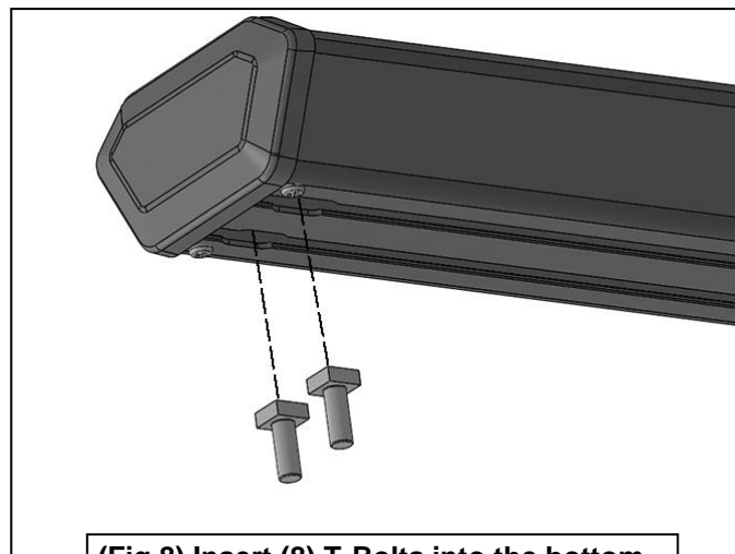
(Fig 8) Insert (8) T-Bolts into the bottom of the Sidebar, (4) per channel
