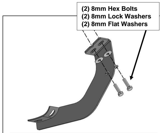
(Fig 5) Attach (1) Passenger/Right Rear Mounting Bracket to the 2nd location
