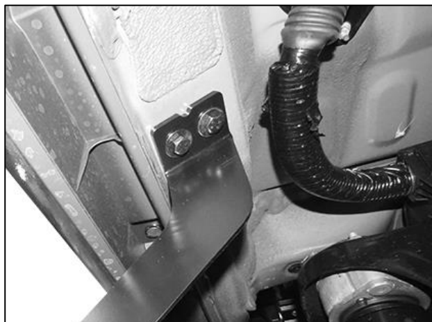
(Fig 8) (1) Passenger/Right Rear Mounting Bracket attached to the rear location
