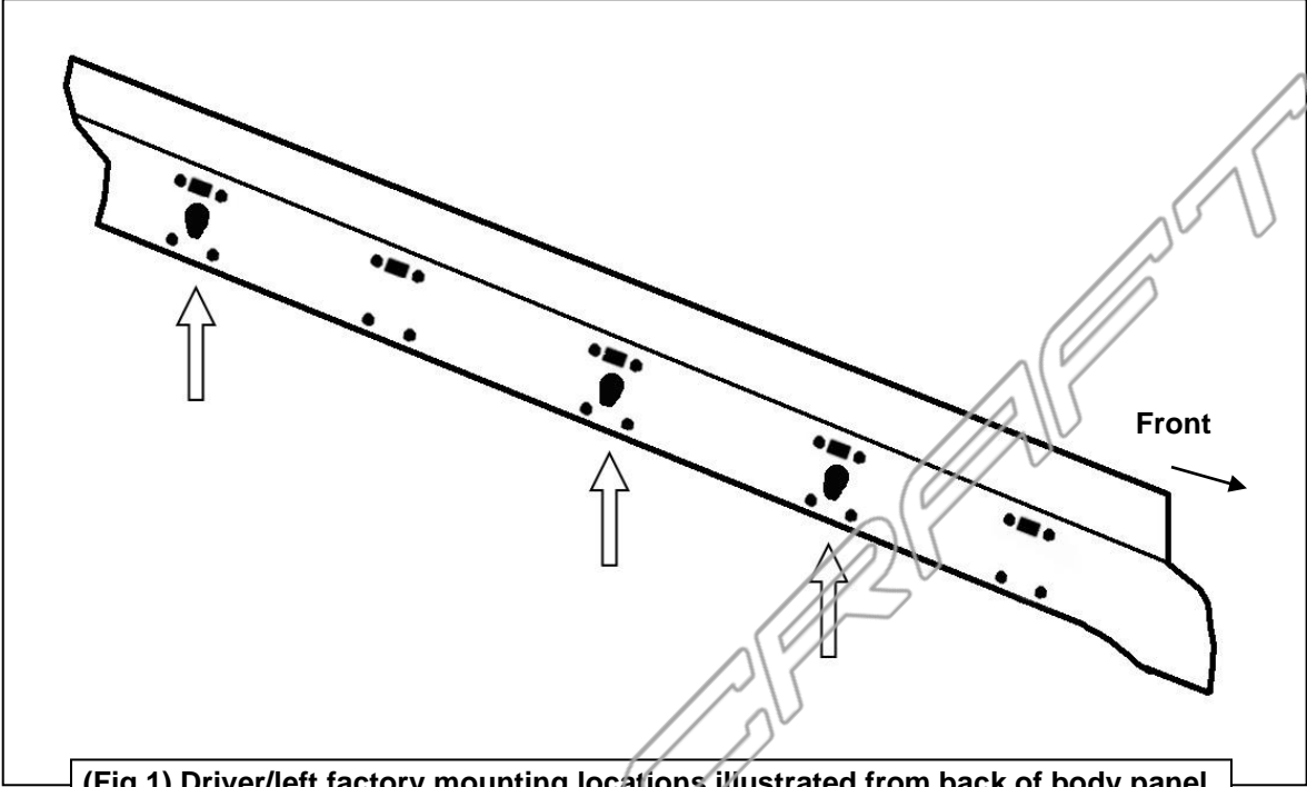
(Fig 1) Driver/left factory mounting locations illustrated from back of body panel
