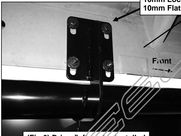
(Fig 6) Driver/left center installed
