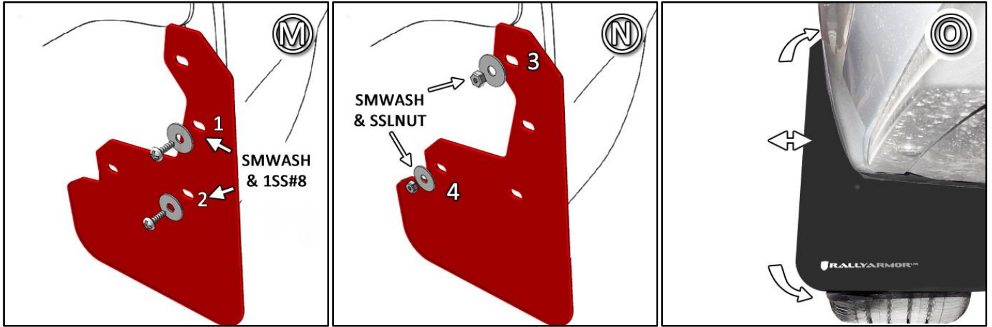
FIGURE O Align flaps to even ground before tightening fasteners until washers just seat against flap.
