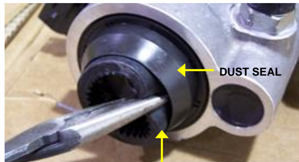
RUBBER SLEEVE
