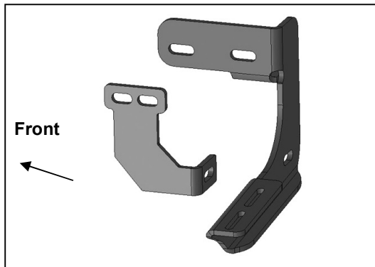
(Fig 6) Driver side front and center Brackets
