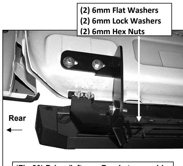
(Fig 20) Driver/left rear Bracket assembly
