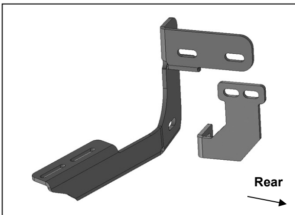
(Fig 16) Driver/Left angled rear Mounting Brackets
