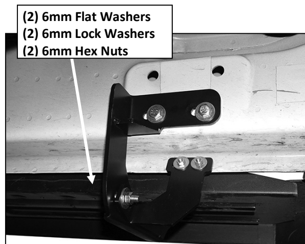
(Fig 19) Driver/left front Bracket assembly
