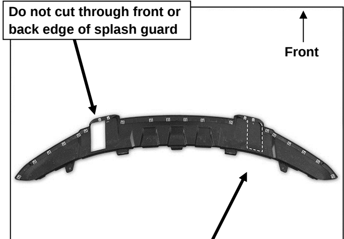
Fig 15) 15-17 models pictured: Hold the splash guard up to the bottom of Frame Brackets. Trace location of Brackets onto back of the plastic cover (dashed line). Cut as required to clear brackets
