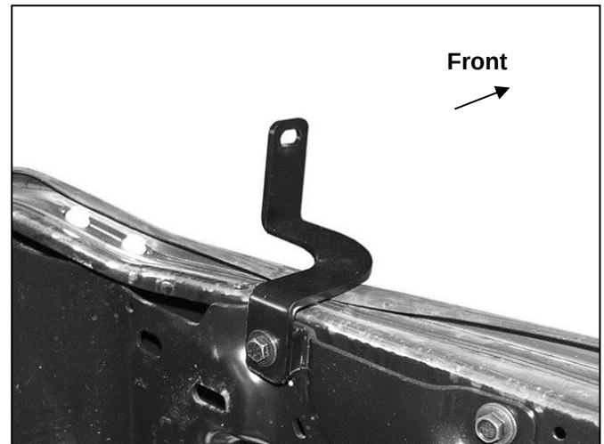
(Fig 21) 2018 models: Attach Top Support Bracket to back of bumper bracket
