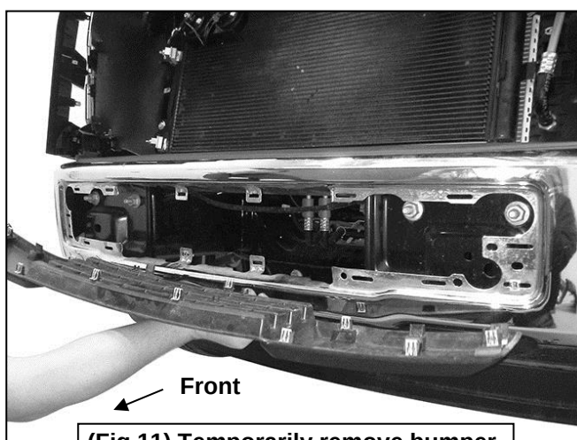
(Fig 11) Temporarily remove bumper pad. Grille removed for instruction purposes only, do not remove grille
