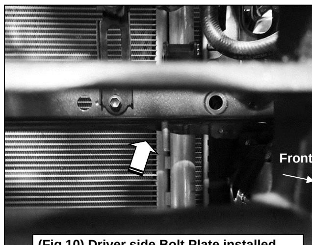
(Fig 10) Driver side Bolt Plate installed
