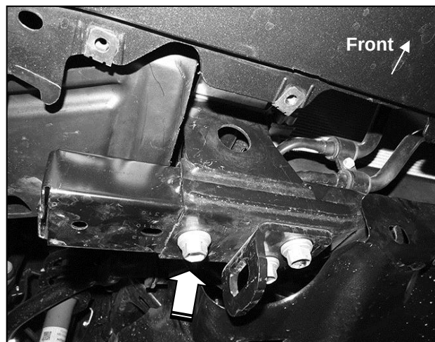
(Fig 2) Remove factory hex bolt (arrow)
