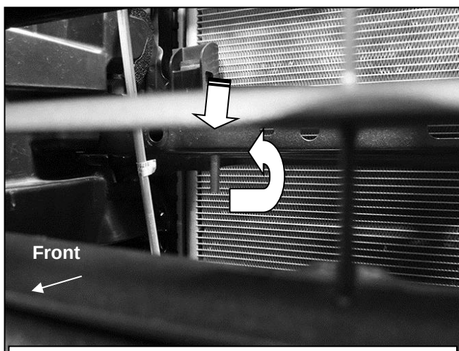
(Fig 9) Insert Bolt plate (arrow) into back of radiator cross support and down through hole in bottom (passenger side pictured through bumper)
