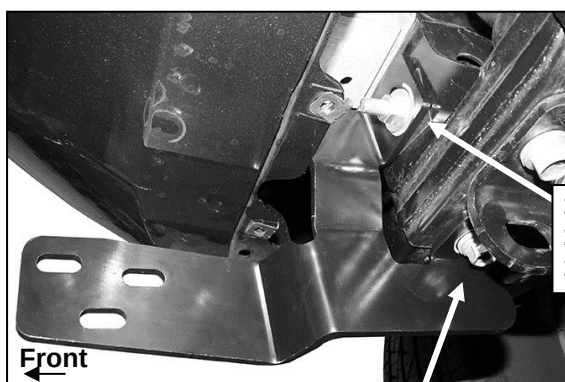
(Fig 5) Reuse factory hex bolt to attach Frame Bracket to bottom of cross-member
