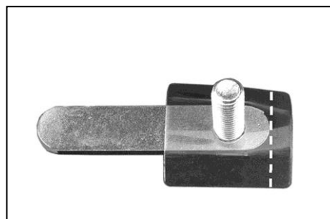
(Fig 12) Bend sides of Plastic Washer up around Bolt Plate. If necessary, use scissors to cut off overhanging plastic. Cut washer on Bolt Plate installation only
