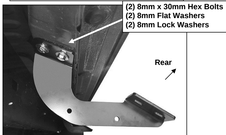
(Fig 11) Passenger side rear Bracket installed
