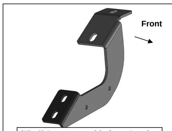
(Fig 2) Passenger side front Bracket
