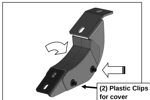
(Fig 4) Push center pin in to expand Clip in Bracket
