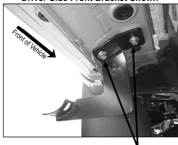
Driver Side Front Bracket Shown
