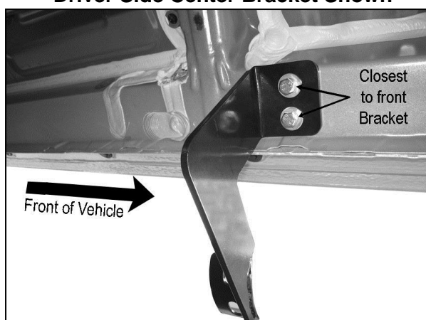
Driver Side Center Bracket Shown
