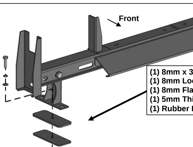
(Fig 12) Installation of Roof Bracket to roof for Transit illustrated
