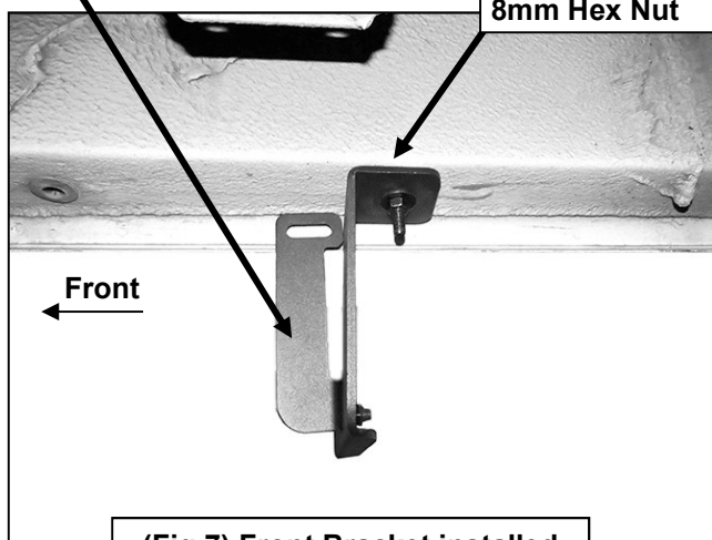
(Fig 7) Front Bracket installed
