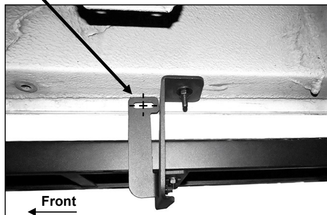
(Fig 10) Mark and drill hole through pinch weld. Attach top of Driver/left front Support Bracket to back of pinch weld. Reinstall Running Board
