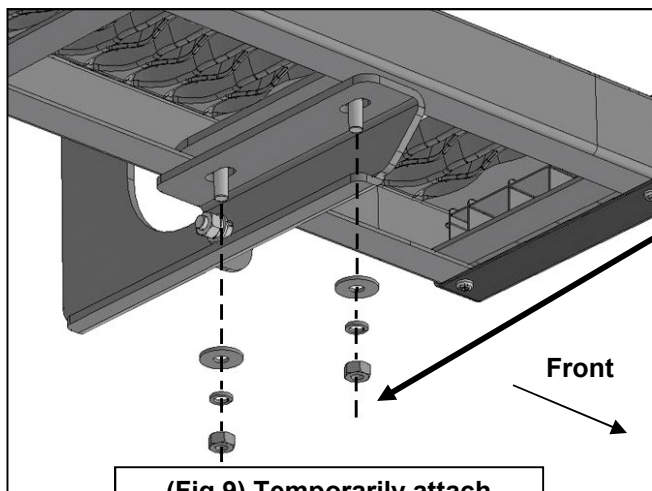
(Fig 9) Temporarily attach Running Board to Brackets
