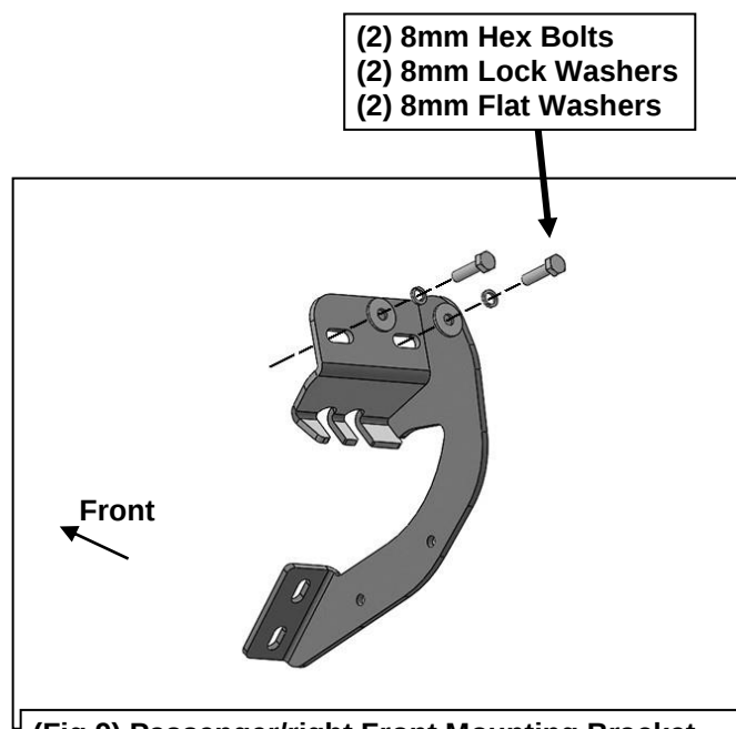
(Fig 9) Passenger/right Front Mounting Bracket illustrated for models with threaded inserts
