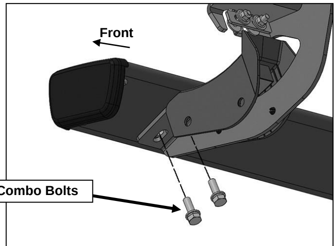
(Fig 14) Attach the Passenger/Right SE5 Sidebar to the Mounting Brackets
