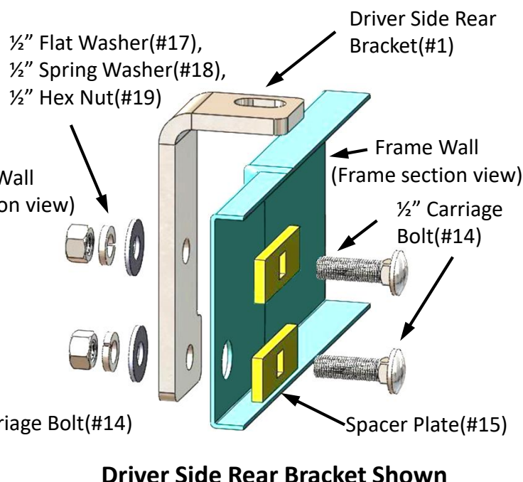
Figure: 4B
