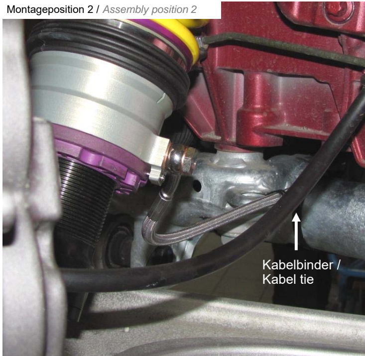
Montageposition 2 / Assembly position 2
