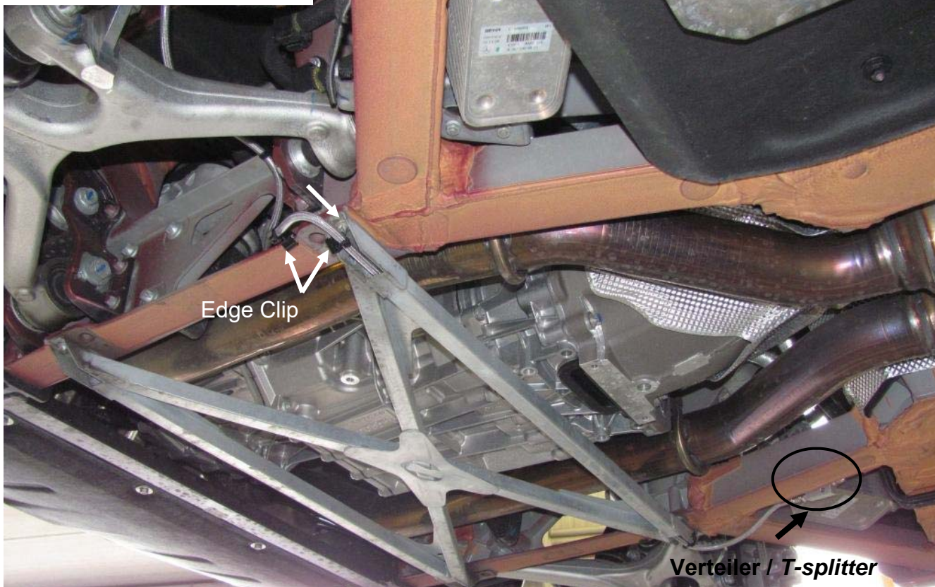
Montageposition 4 / Assembly position 4
