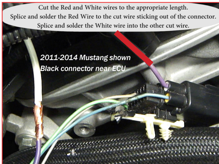
Use the wire Extension kit to extend the Red/White 10 gauge wires. Install the wire loom to protect the wires.
