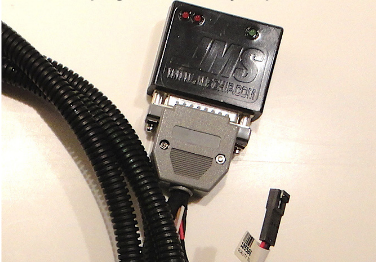
ID the Map Sensor Connectors: Two Green wires
