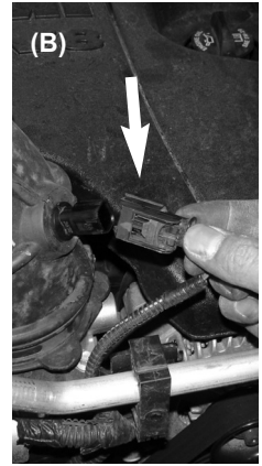
Figure 5(B) Unclip harness from from air temp sensor.
