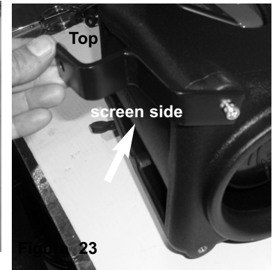
Figure 23 Now install the bracket p/n:20108 to the front of the powerflow box.
