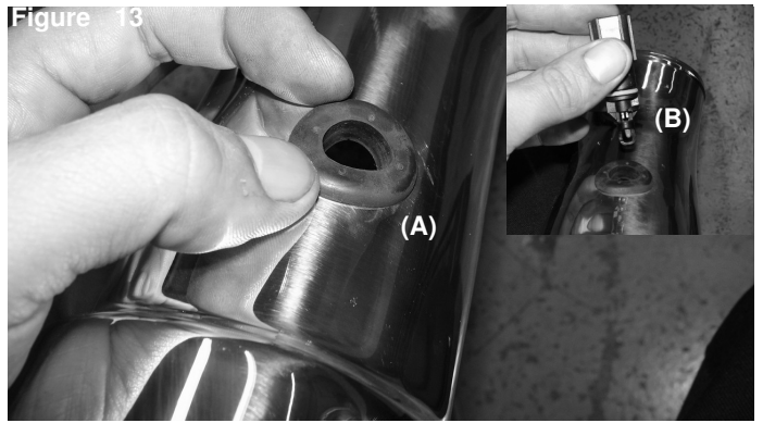
Figure 13 Locate the sensor grommet in this kit and press it into the pre-drilled hole as shown above (A). Continue to press the sensor grommet into the pre-drilled intake hole until the top sits flush with the intake out side radius (B). Install the temperature sensor into the grommet.
