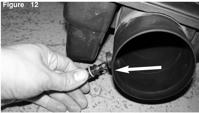
Figure 12 Carefully turn then pull out the temperature sensor out of resonator box.
