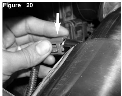
Figure 20 Connect the temperature sensor harness.
