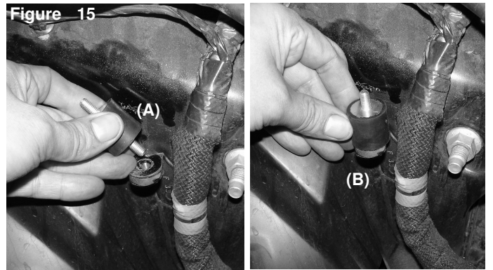
Figure 15 A) Install the provided M6 vibra mount to the threaded insert located next to the radiator reservoir. B) Secure and tighten the M6 vibra mount.
