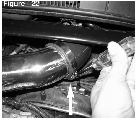
Position the elbow hose for the best possible fit. Tighten the clamp using 8mm nut driver.
