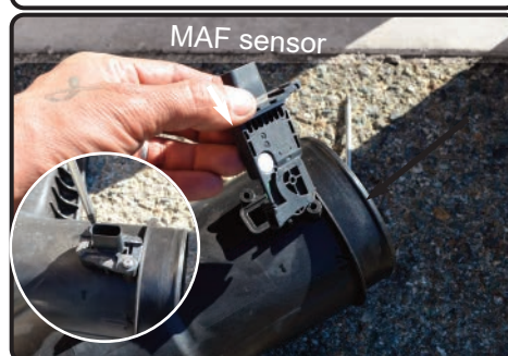
11. Using a T20 torx bit remove the two screws holding in the MAF sensor and remove the MAF sensor.
