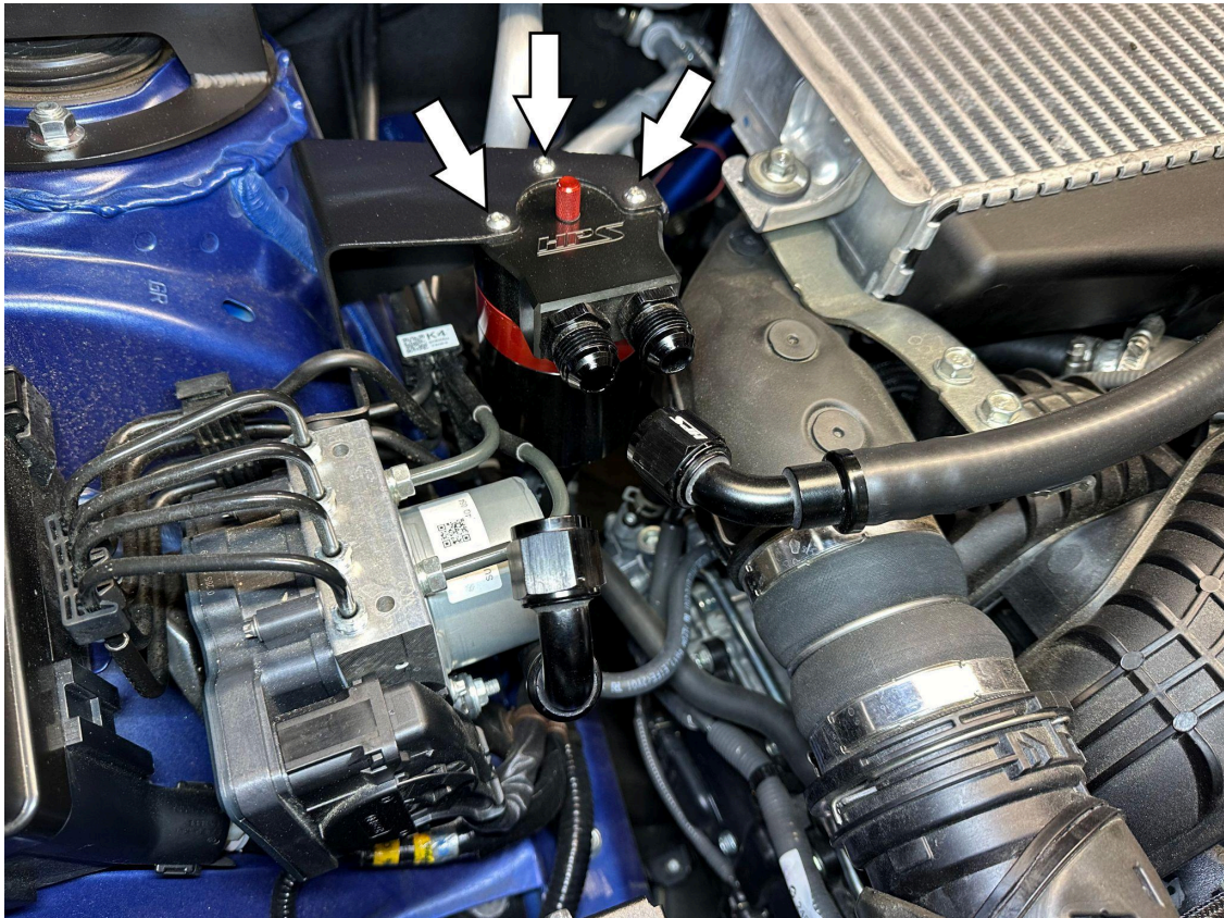
17. Mount the HPS oil catch can to the oil catch can bracket using the three provided M5 bolts.
