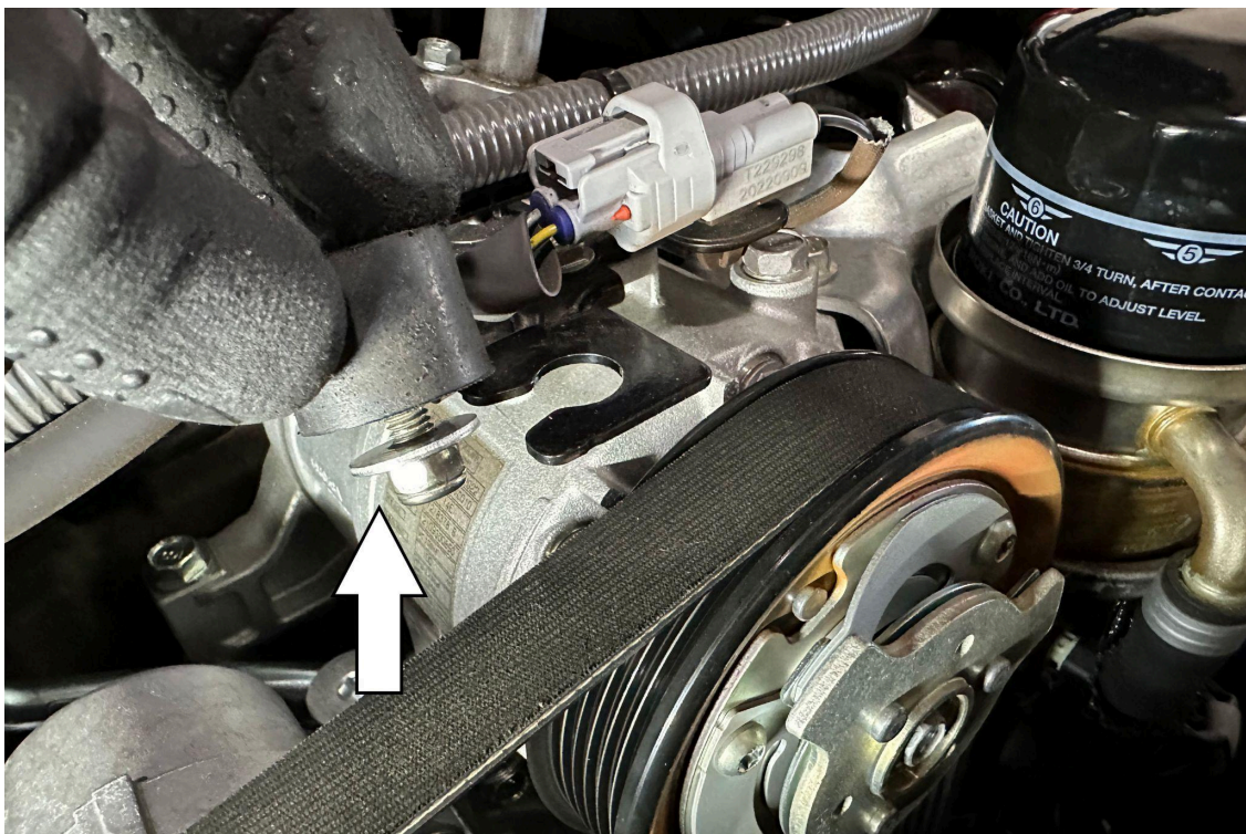
4. Pre-assemble the provided rubber vibration mount with an M6 flat washer and M6 Nylock Nut as shown in the image above.
