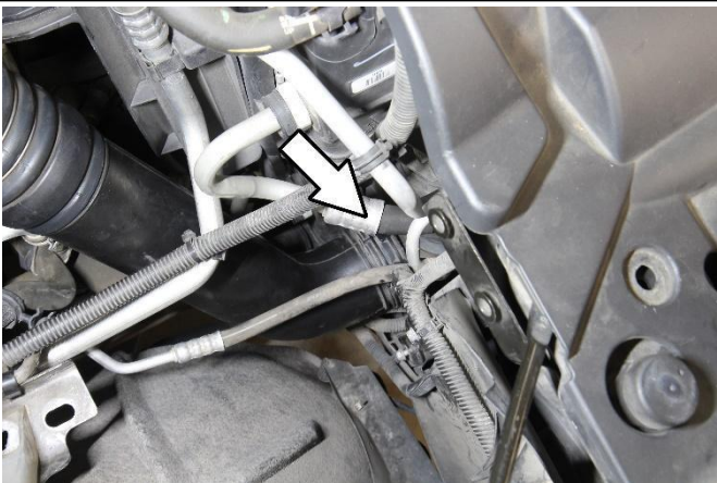
10. Using a flat head screwdriver, rotate the locking mechanism counterclockwise to release the charge pipe from the intercooler.
