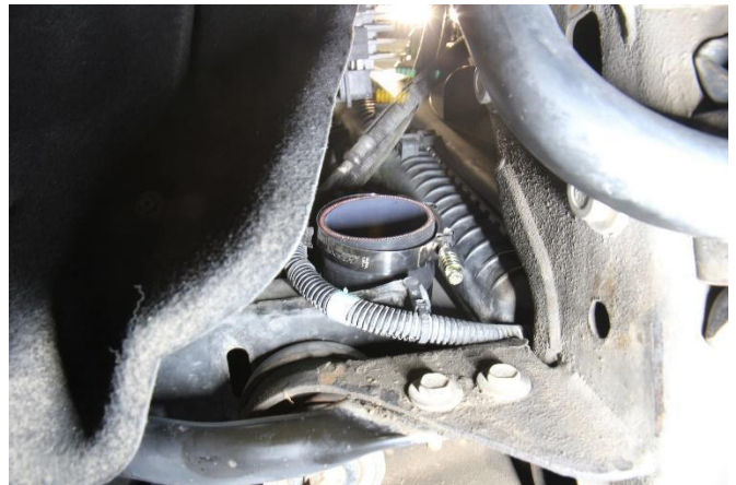
23. Install the other reducer coupler, along with the provided T-bolt clamps onto the intercooler inlet.
