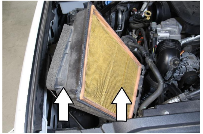
7. Gently lift up and disconnect the lower air box assembly from the rubber grommets. Remove the lower air box assembly from the vehicle.
