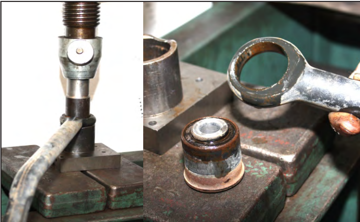
Use a hydraulic press to remove the original bushings, including the outer metal shell the rubber is bonded to.
