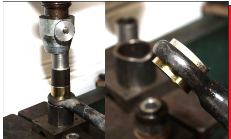
Press in the supplied shells into the track bar and center them evenly.
