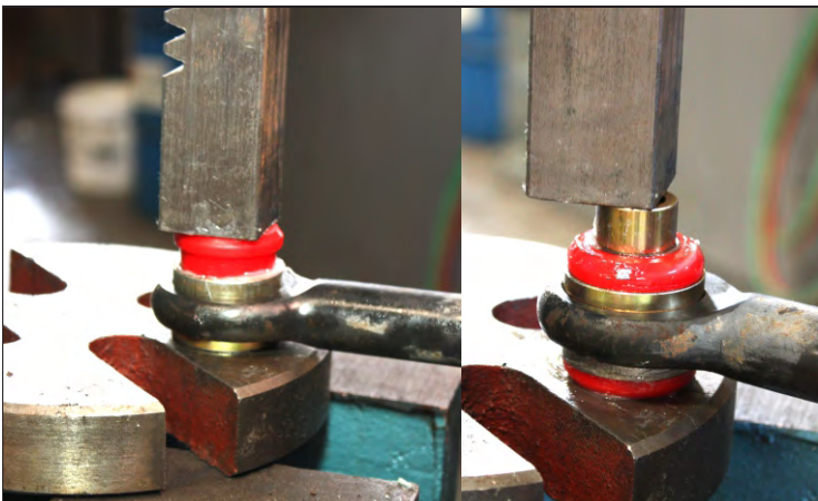
Press in the Energy Suspension bushings 7141, then grease the sleeve and press into the bushings.
