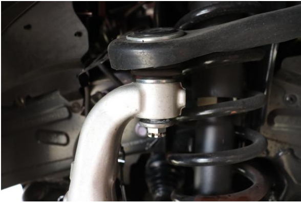
7. Loosen but do not remove the upper control arm ball joint nut.
