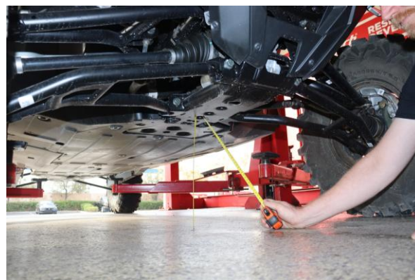
Step 22. Measurement shown from level floor surface to front skid plate 355mm (14" inches).
