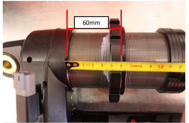
Step 16. Set the preload collar to 60mm ( 2 23/64 IN) from the bottom of the Resi crossover to the bottom of the preload collar
